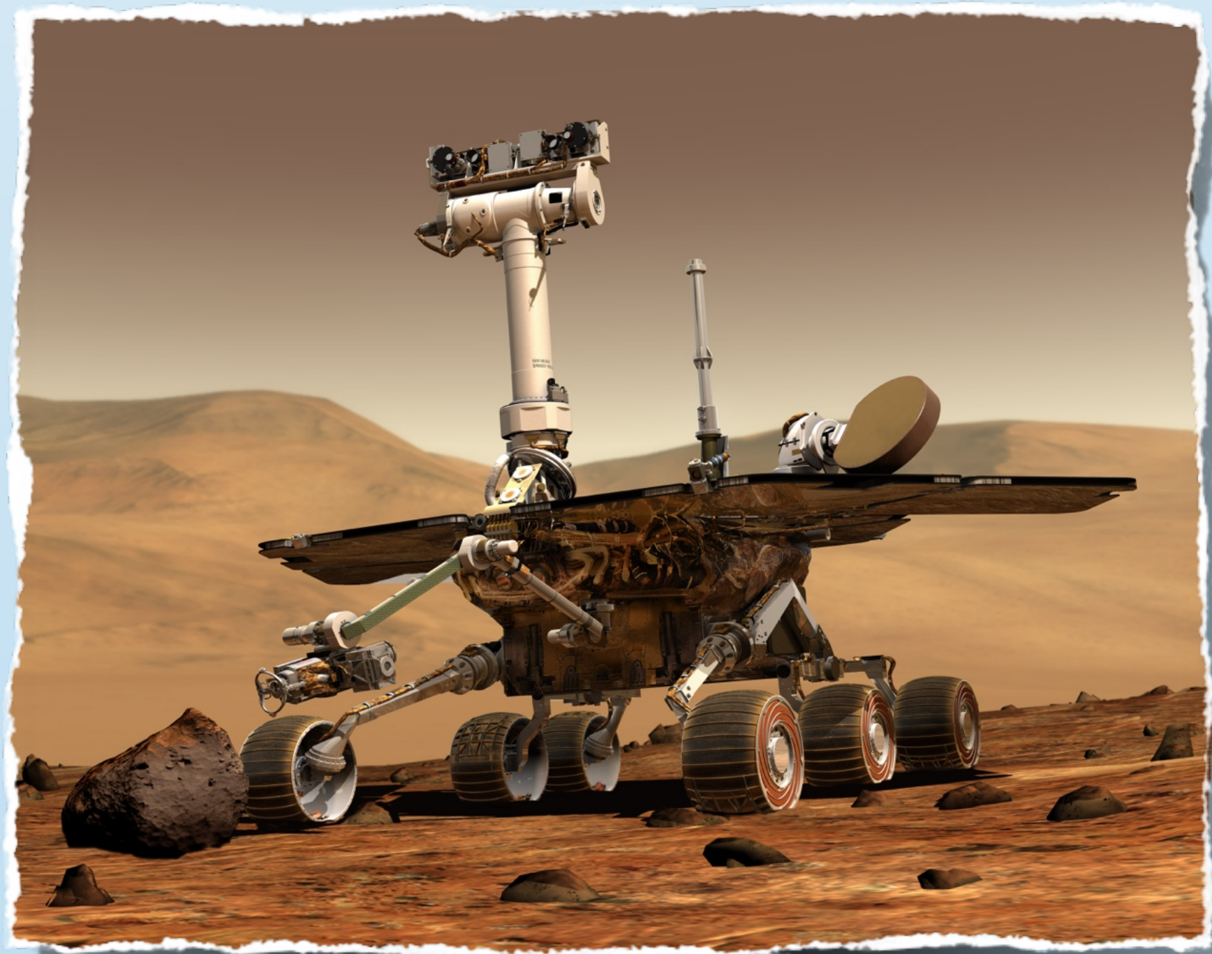
Source: NASA/JPL-Caltech 2012
